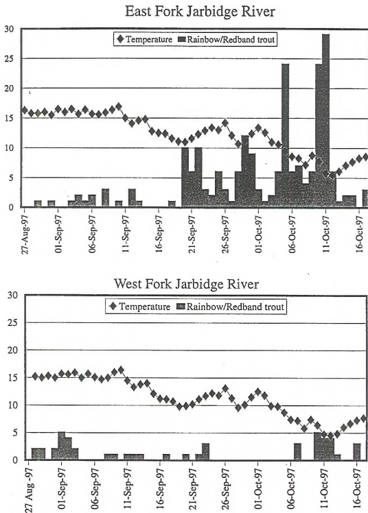
Figure 2. Number of rainbow/redband trout and daily mean water temperature (C) sampled at traps on the East Fork and West Fork, Jarbidge River.
